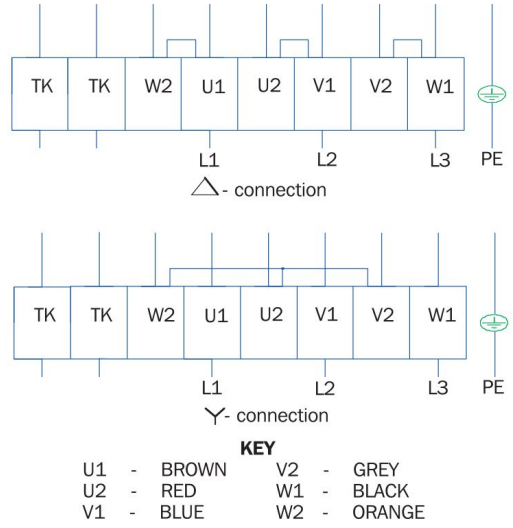
Motor/Fan details
